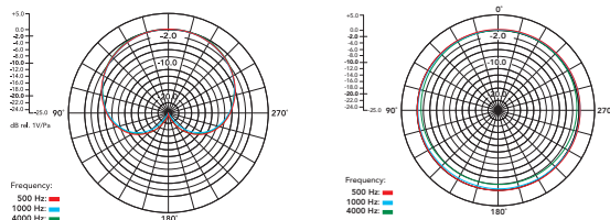
CARDIOID CAPSULE
